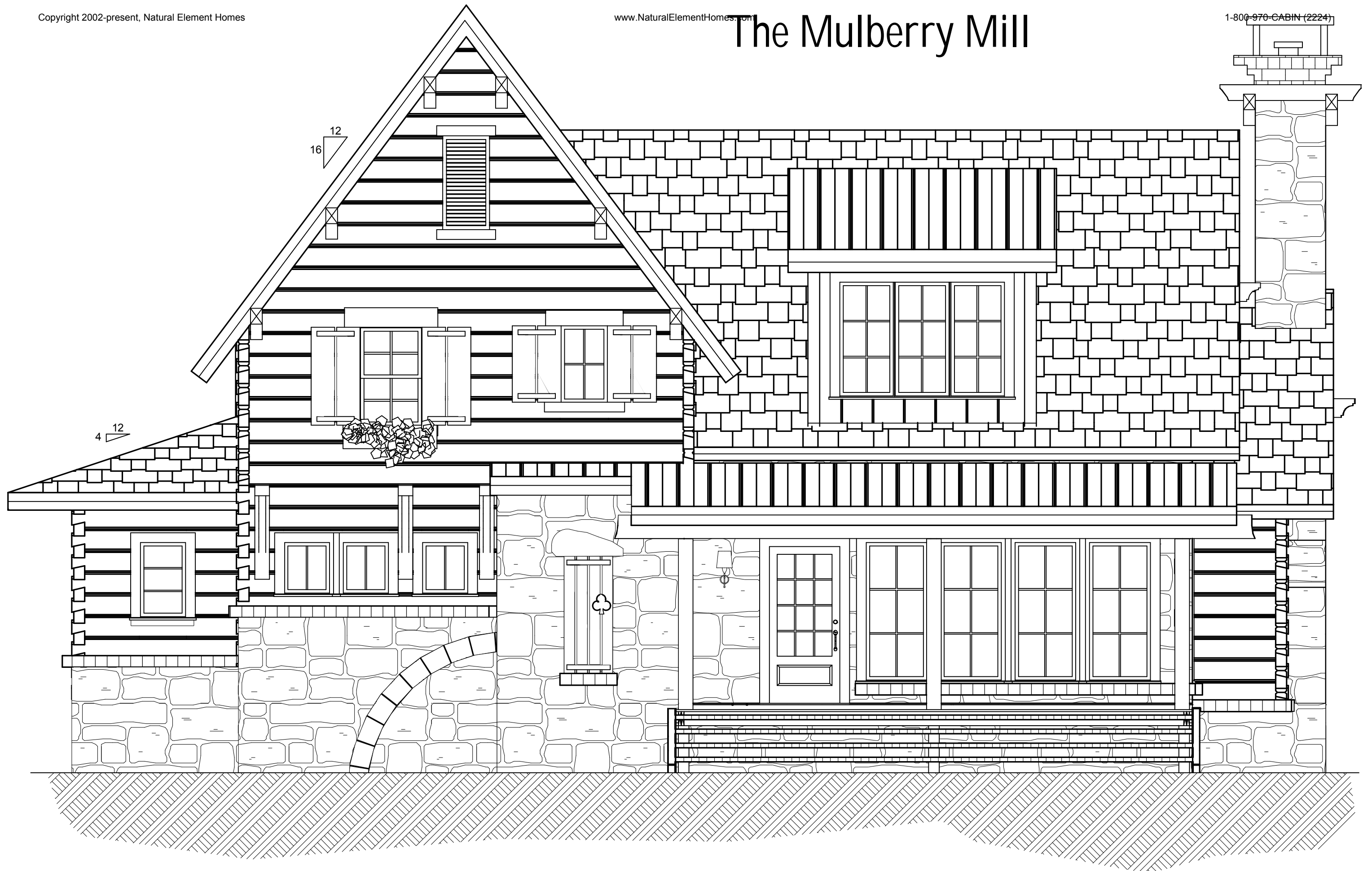
FRONT ELEVATION
